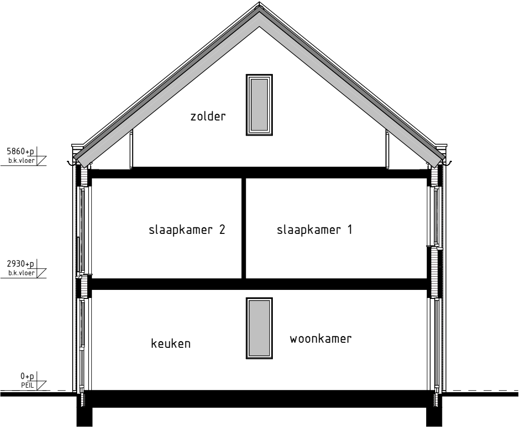
DOORSNEDE K1sp-K1sp
