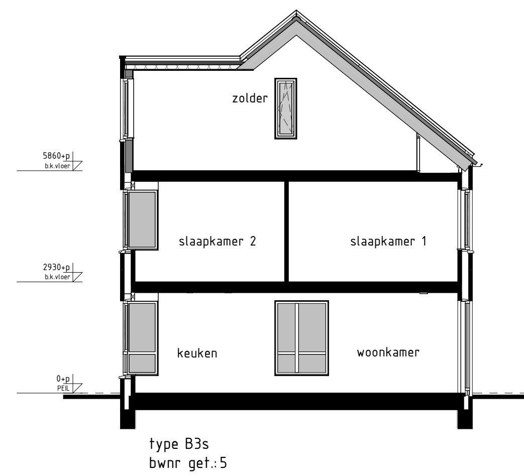
DOORSNEDE B3s-B3s
