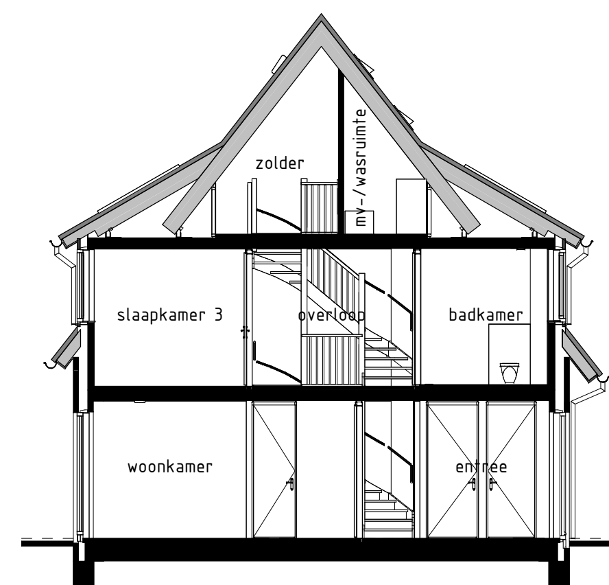
type S1sp, S2, T1 bwnr get.:02 bwnr gesp.:03, 04, 05 DOORSNEDE S1sp-S1sp 1:50
