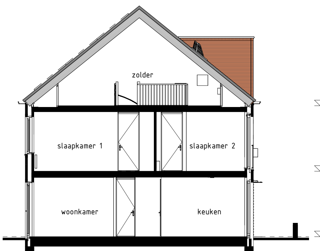
type A1sp, B4sp bwnr get.:548, 550, 551, 552 DOORSNEDE A1sp-A1sp 1:50
