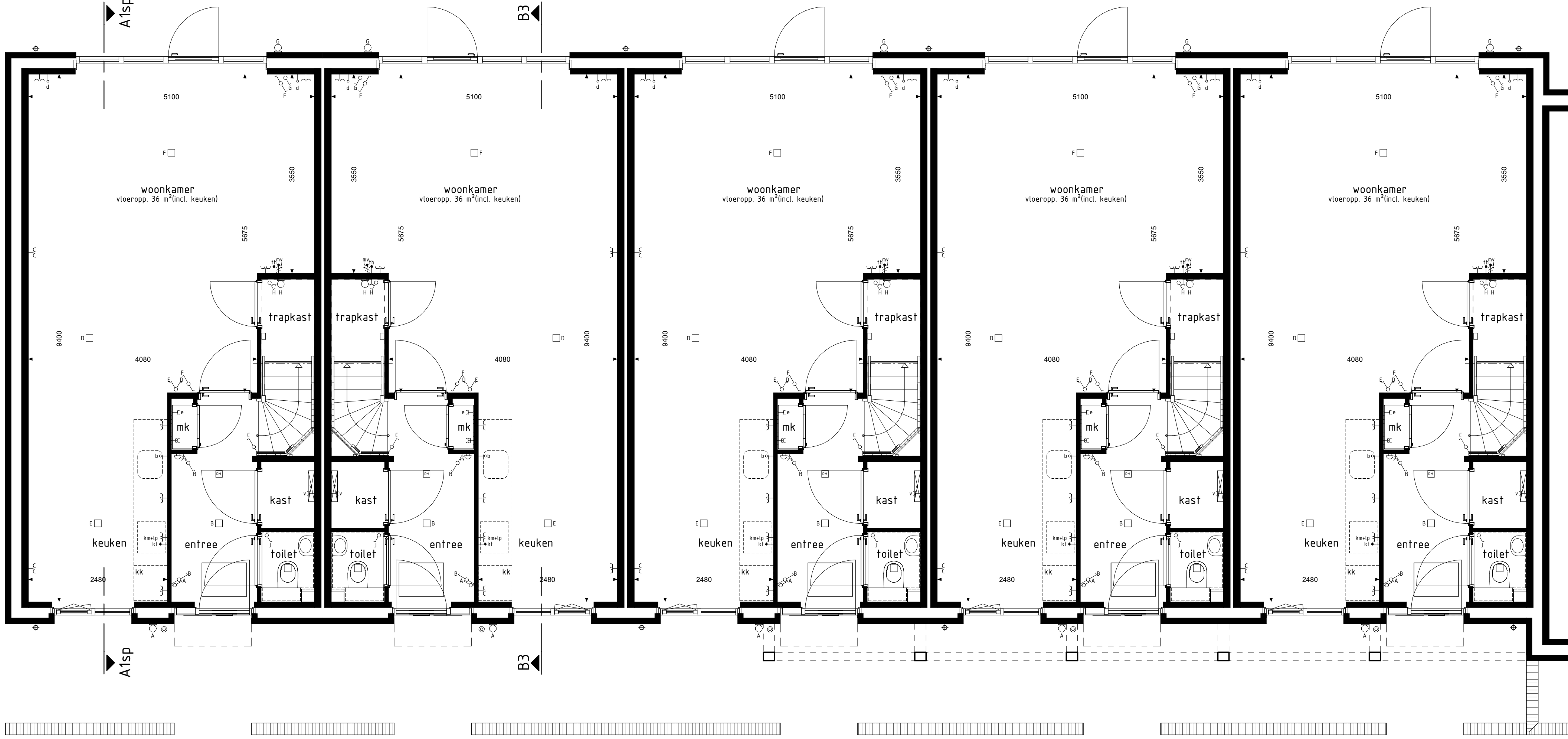
type A1sp bwnr get.:548 type B3 bwnr get.:549 type B4sp bwnr get.:550 type B4sp bwnr get.:551 type B4sp bwnr get.:552 BEGANE GROND 1:50
