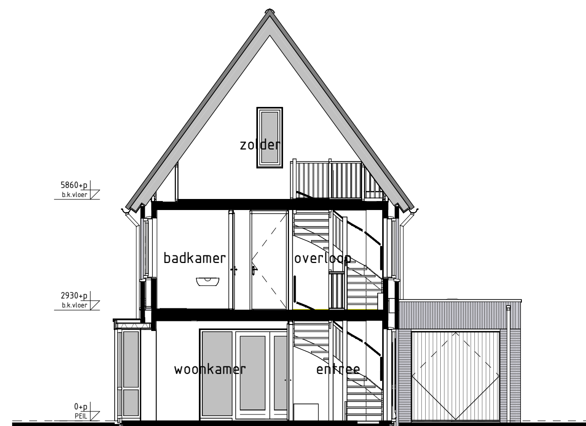
type N1sp bwnr get.:49 DOORSNEDE N1sp-N1sp
