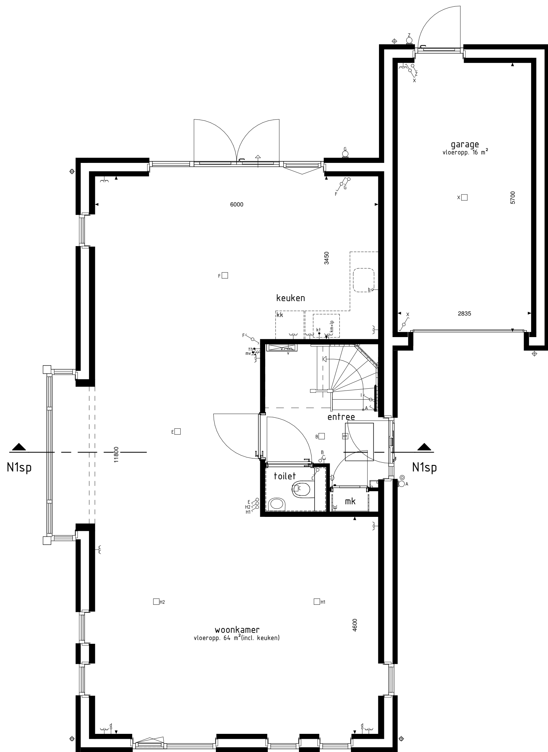
type N1sp bwnr get.:49
