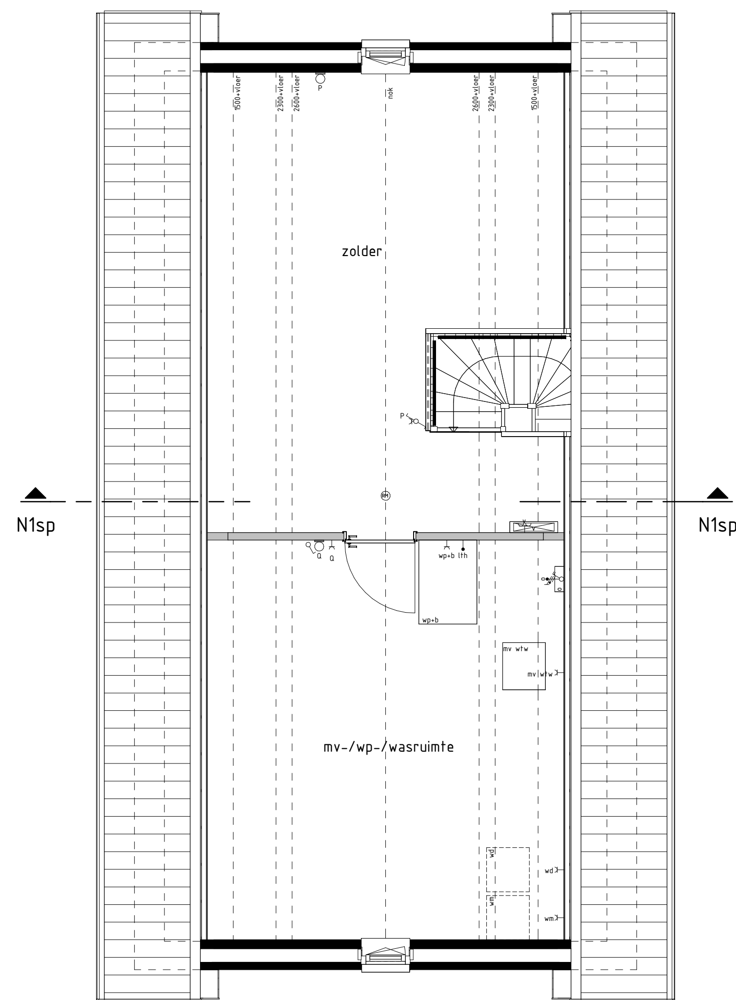
type N1sp bwnr get.:49
