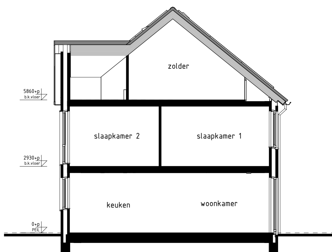
type I1sp bwnr get.:113 DOORSNEDE I1sp-I1sp 1:100
