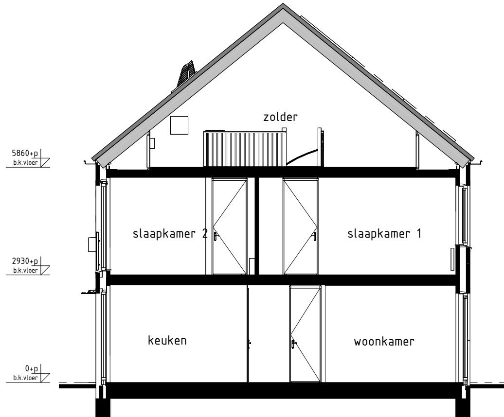
type A2sp, B1, B4 bwnr get.:536, 537, 539 DOORSNEDE B1-B1 1:50
